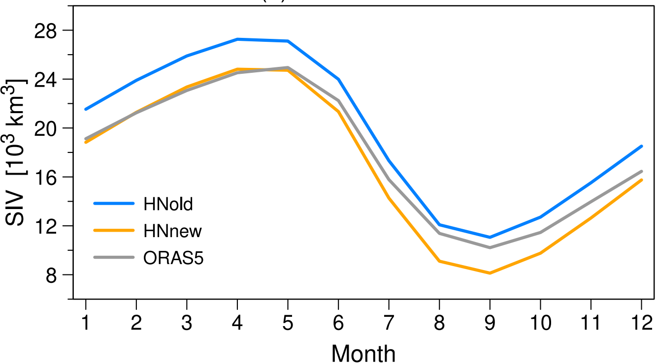
(a) Sea-Ice Volume
