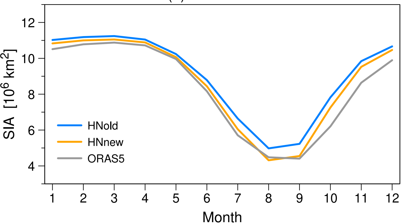
(b) Sea-Ice Area
