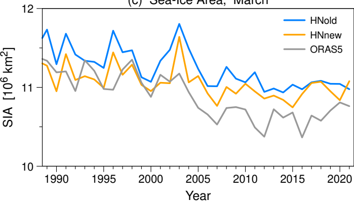
(c) Sea-Ice Area, March
