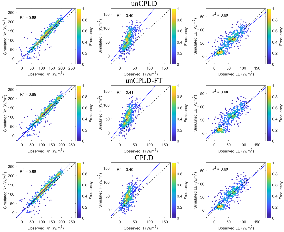
Figure S2. Scatter plots of observed and model simulated daily average surface fluxes (net radiation: R_n , latent heat: LE and sensible heat flux: H ) using the original (uncoupled) T&C (unCPLD), T&C with consideration of FT process (unCPLD-FT) and coupled T&C and STEMMUS (CPLD) model during the non-frozen period, with the color indicating the occurrence frequency of surface flux values.
