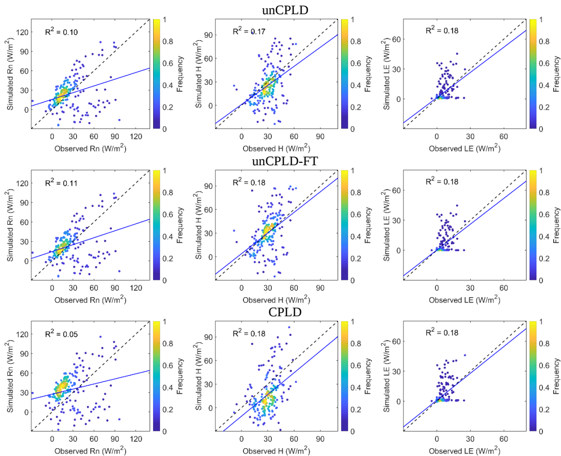
Figure S3. Scatter plots of observed and model simulated daily average surface fluxes (net radiation: R_n , latent heat: LE and sensible heat flux: H ) using the original (uncoupled) T&C (unCPLD), T&C with consideration of FT process (unCPLD-FT) and coupled T&C and STEMMUS (CPLD) model during the frozen period, with the color indicating the occurrence frequency of surface flux values.
